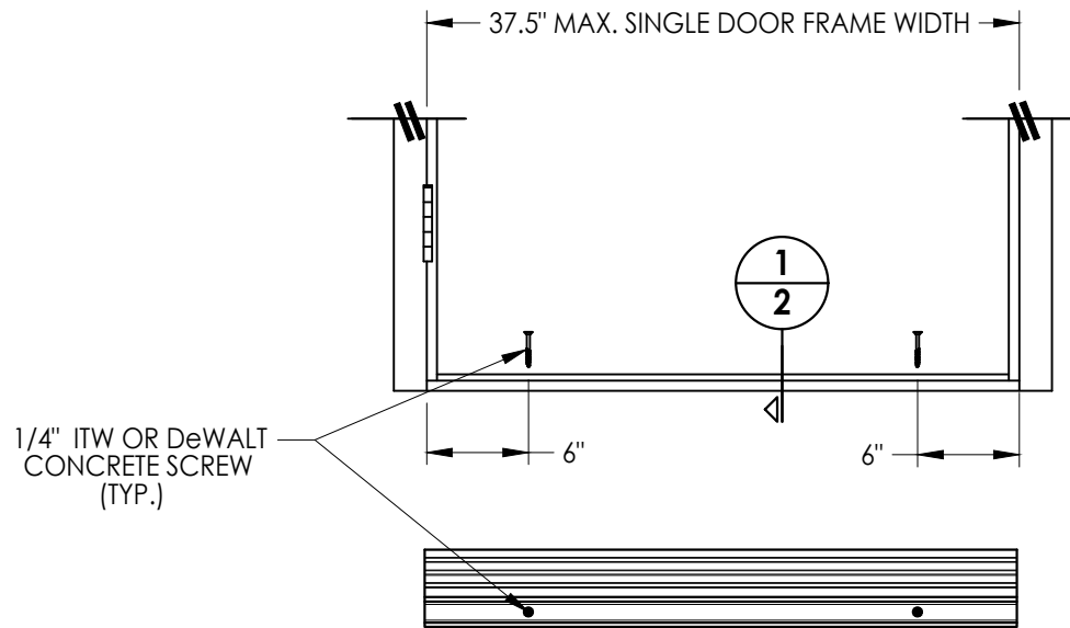
TYPICAL SINGLE DOOR INSTALLATION
