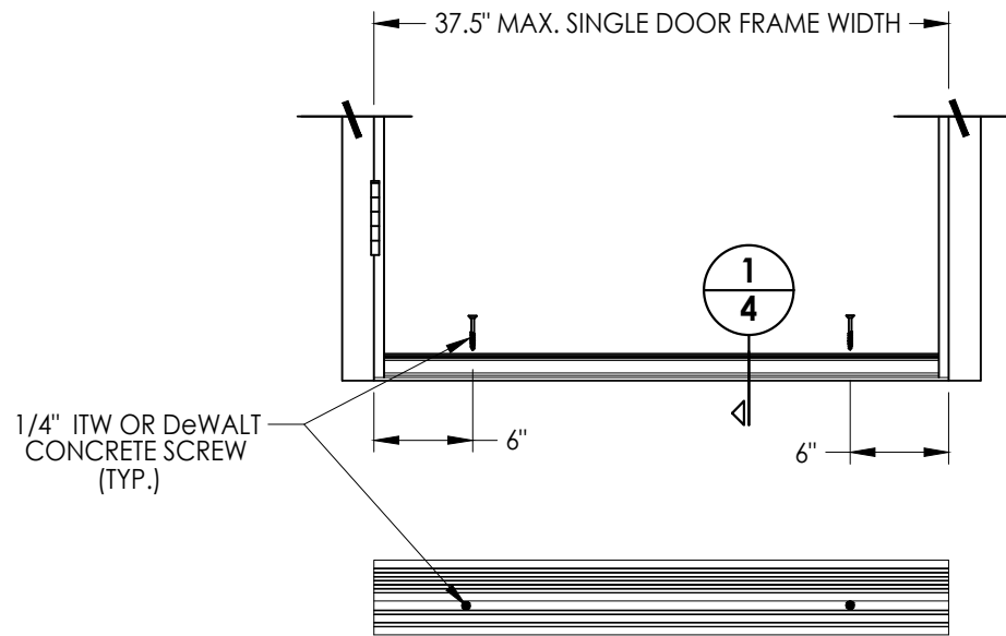
TYPICAL SINGLE DOOR INSTALLATION
