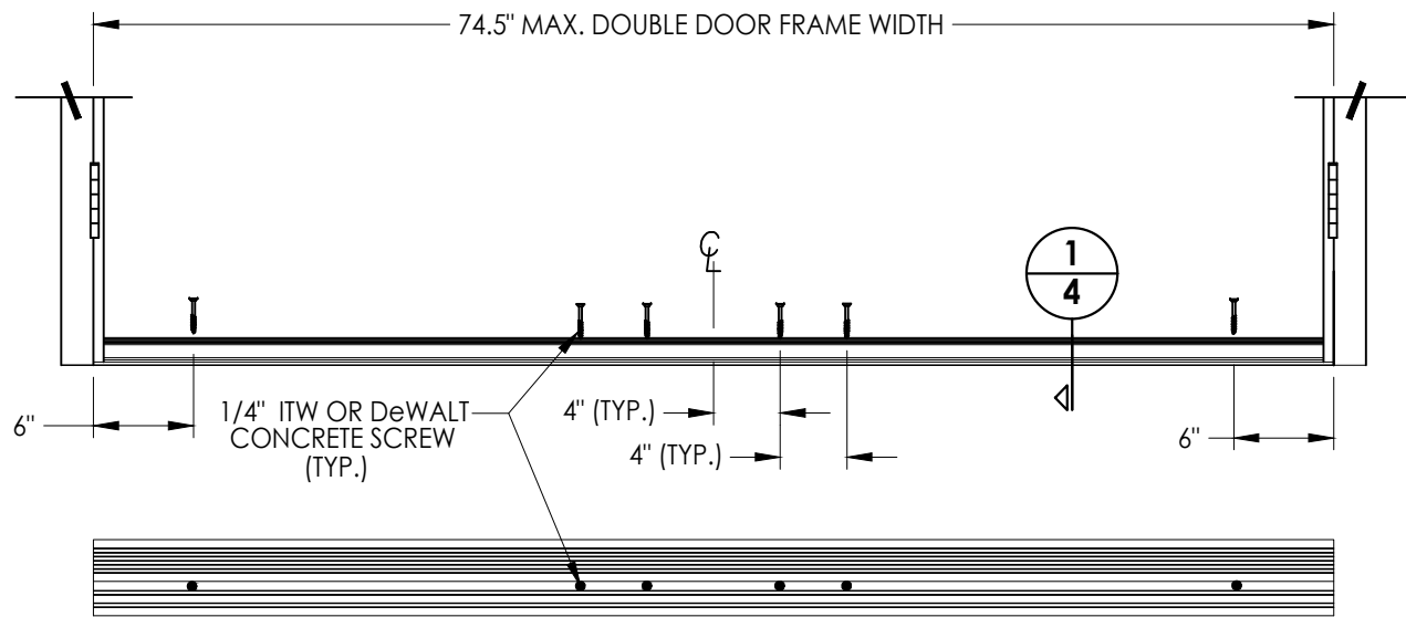
TYPICAL DOUBLE DOOR INSTALLATION
